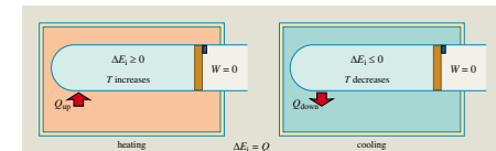
43.2. Characteristics of the energy exchange between gases and the environment during isochoric processes
